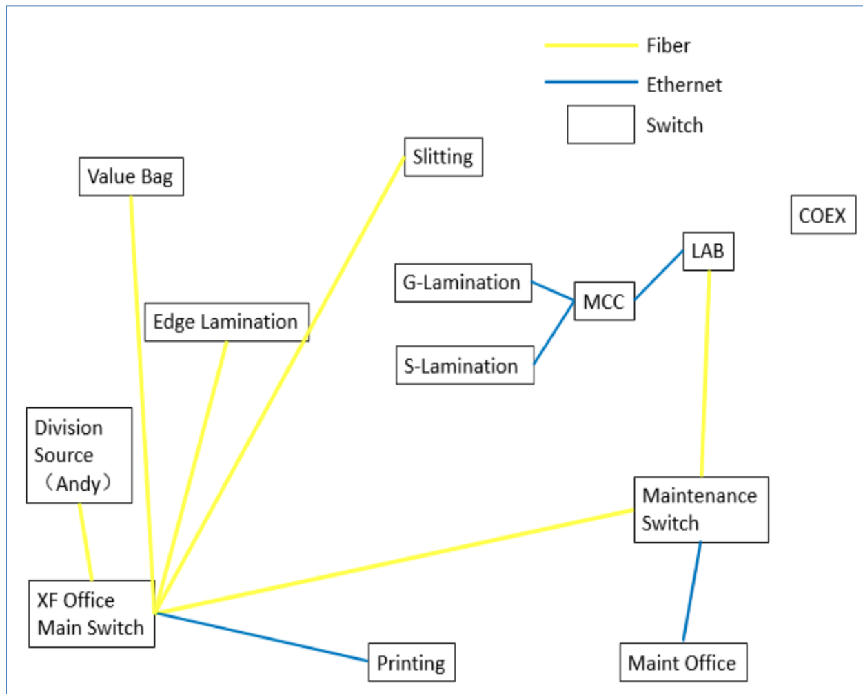
Figure 6.1: XF Network Topology Diagram - XF facility network topology diagram containing yellow fiber-optic links and blue Ethernet connections.
